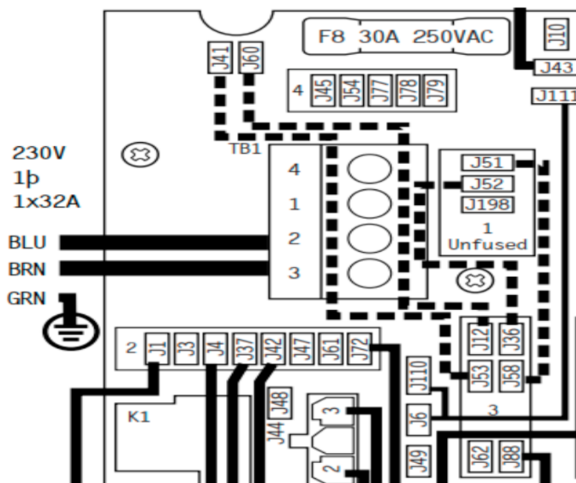
Cablage monophasé (1 x 16amps/32amps)
